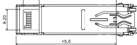
Bottom View
