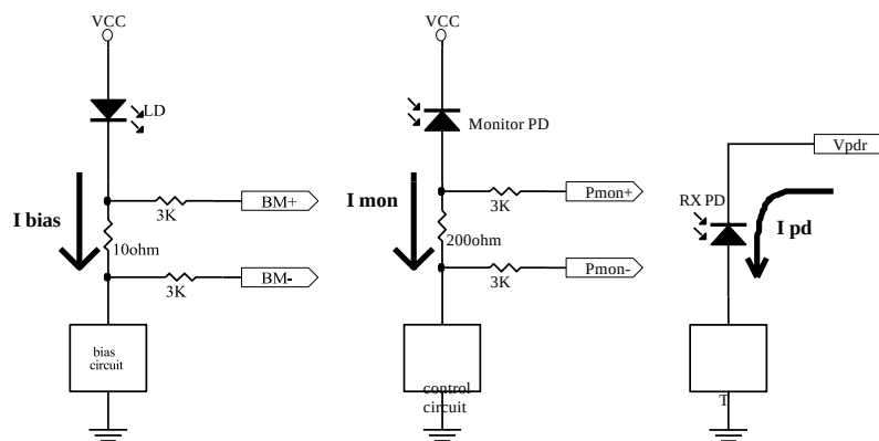
Analogue Monitoring Function Connections
